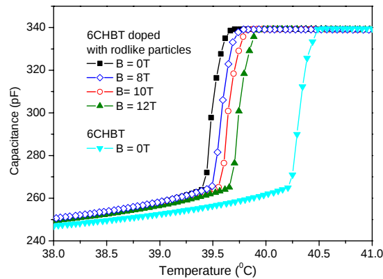
Figure 2: Capacitance vs. temperature for undoped 6CHBT and 6CHBT doped with rodlike magnetic particles measured at different magnetic fields.
