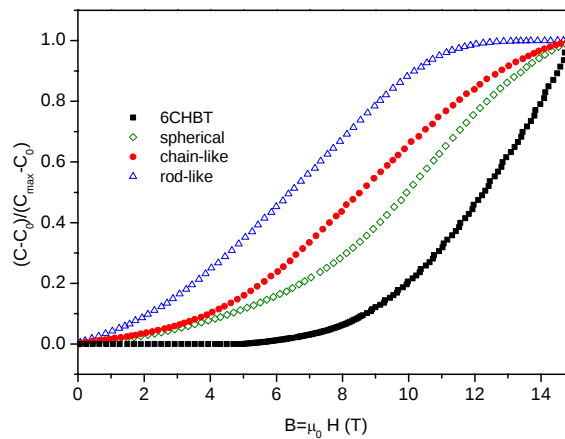
Figure 1: Reduced capacitance dependence of undoped 6CHBT and 6CHBT doped with spherical particles, chain-like particles and rod-like particles on external magnetic field measured at U_B = 10\text{V} ( C_0 and C_{\text{max}} are the capacitance at B=0 and at B which restores the planar alignment, respectively).
