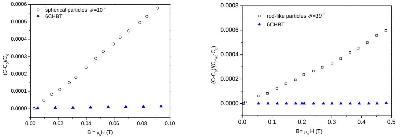
Figure 3: Reduced capacitance versus magnetic field for undoped 6CHBT and for 6CHBT doped with spherical particles and rod-like particles.
