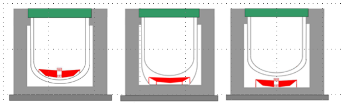
Figure 1: Three options for core catcher location.
